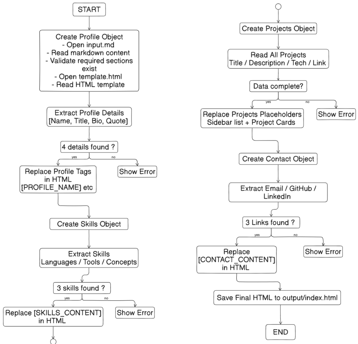
Flow Diagram of C++ Program
